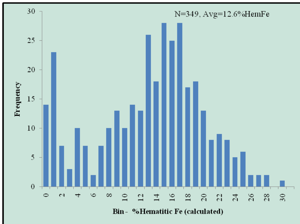
Figure 7. Histogram for %HematiticFe (calculated) in Rockex 2008 program drillhole samples
