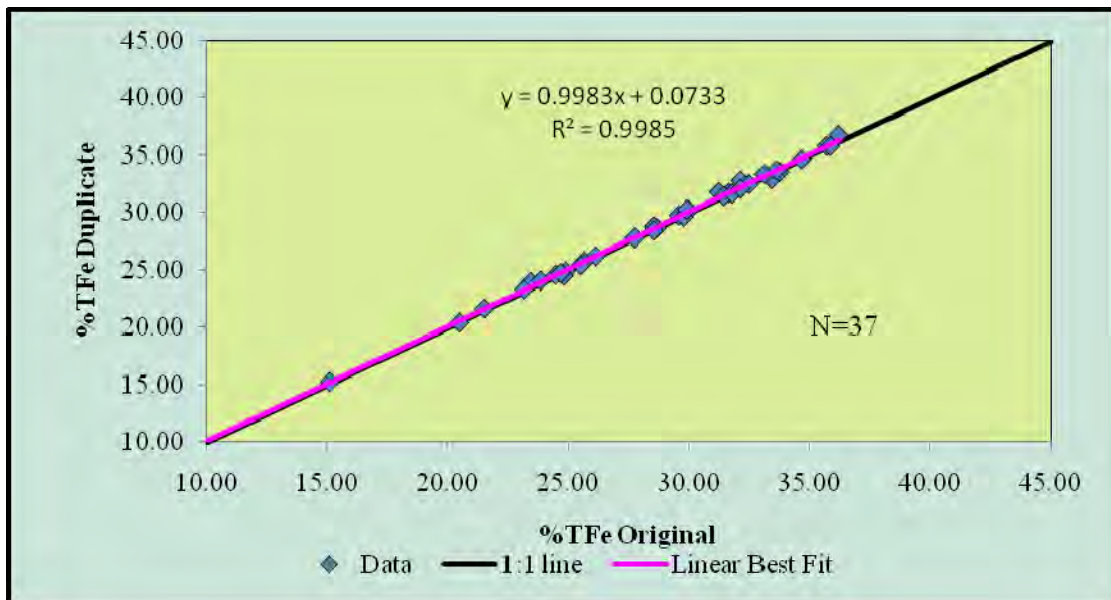
Figure 25. %TFe for Analytical Duplicate vs. Original
