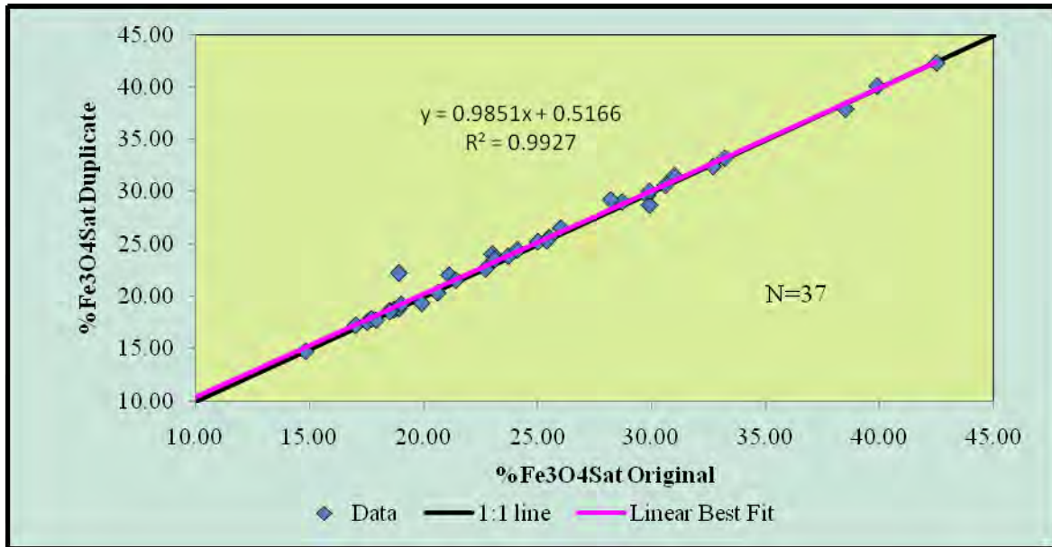
Figure 26. %Fe 3 O 4 for Analytical Duplicate vs. Original
