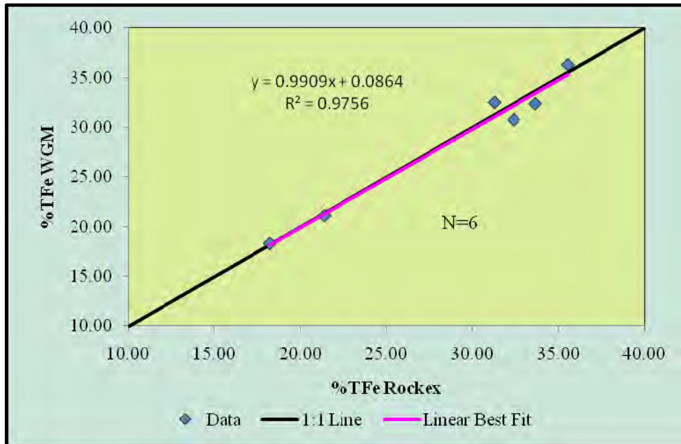
Figure 28. %TFe for WGM Independent Samples vs. Rockex Original
