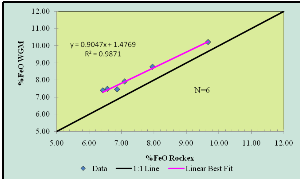
Figure 30. %FeO for WGM Independent Samples vs. Rockex Original
