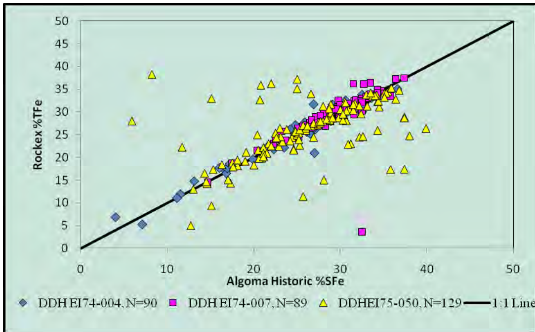
Figure 18. Rockex %TFe assays vs. Historic Algoma %SFe assays for equivalent samples
