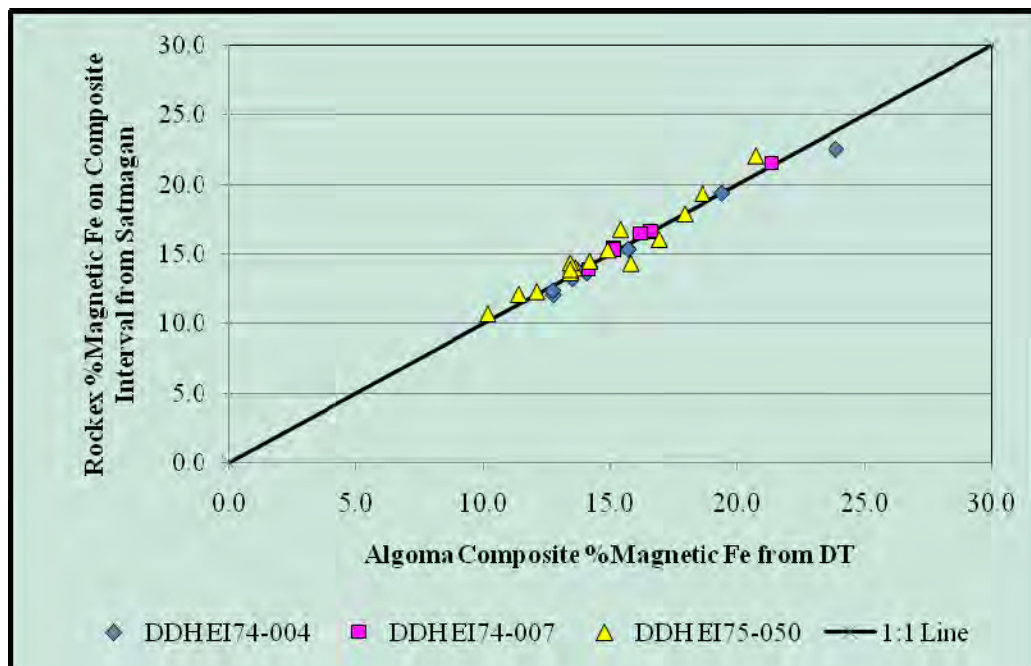
Figure 19 %Magnetic Fe for Rockex samples vs. Algoma Composites
