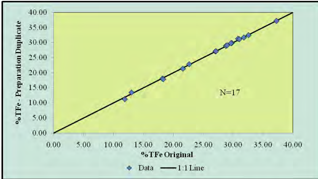
Figure 27. Analytical Results for Preparation Duplicates 2010 historic drill core re-sampling program
