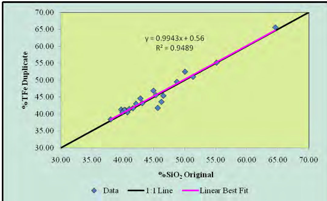
Figure 23. %SiO 2 for Second Half Core Duplicate vs. Original
