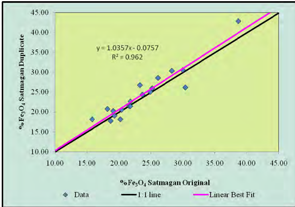
Figure 21. %Fe 3 O 4 for Second Half Core Duplicate vs. Original
