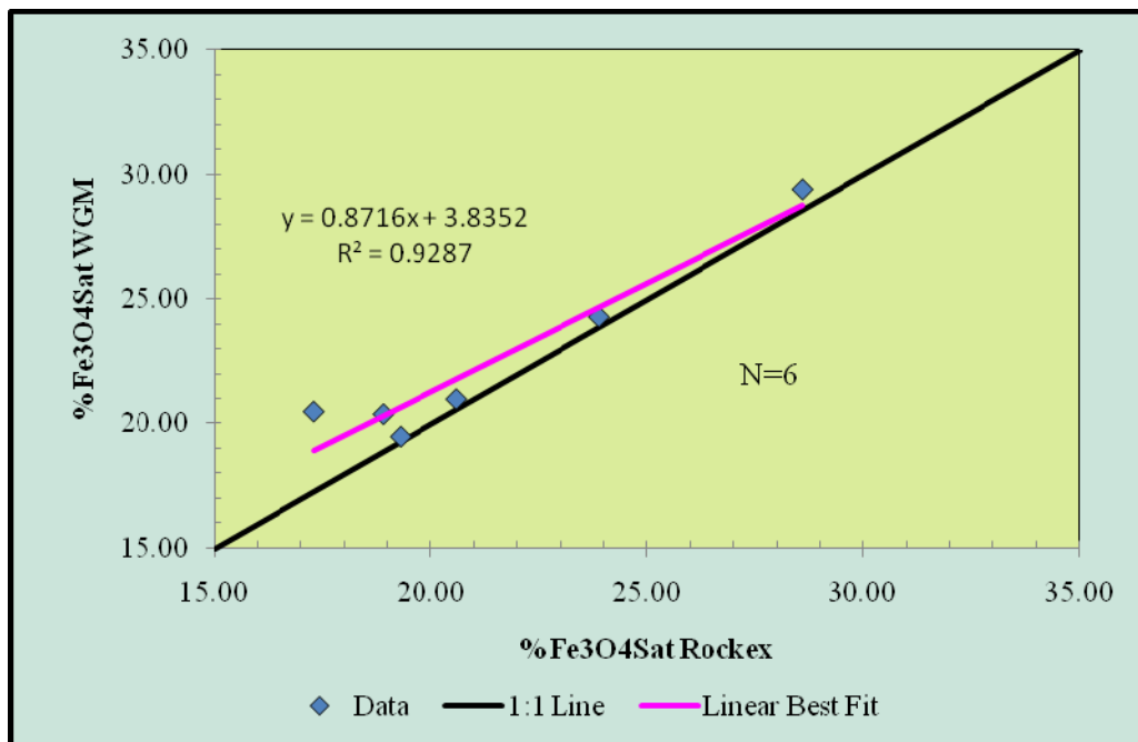
Figure 29. %Fe 3 O 4 Satmagan for WGM Independent Samples vs. Rockex Original
