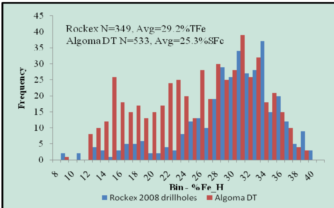
Figure 5. Histogram for %TFe in Rockex 2008 program drillhole samples and %SFe for historic Algoma drillhole sample composites
