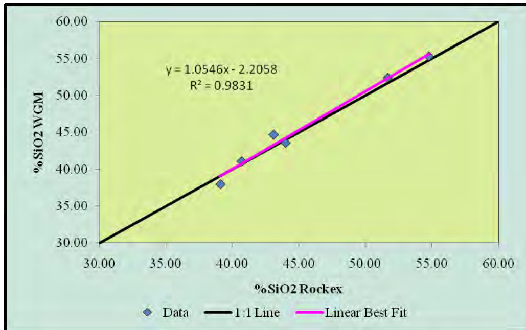
Figure 31. %SiO 2 for WGM Independent Samples vs. Rockex Original
