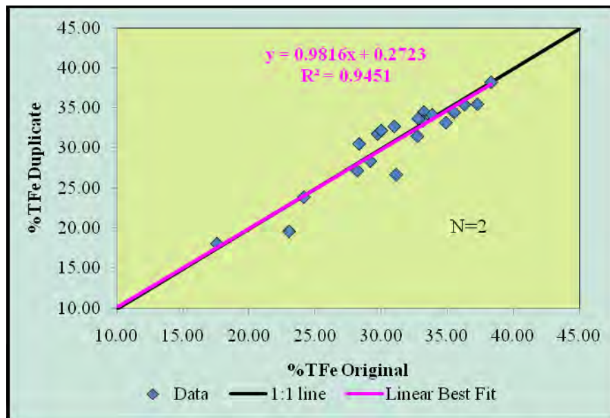
Figure 20. %TFe for Second Half Core Duplicate vs. Original
