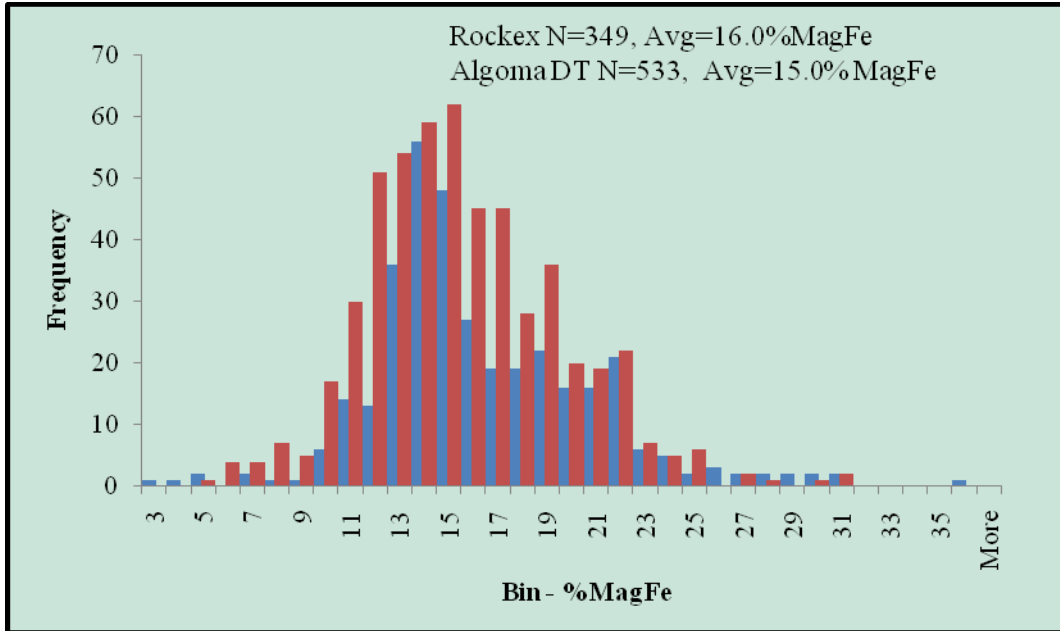
Figure 6. Histogram for %MagneticFe in Rockex 2008 program drillhole samples and Algoma historic drillhole composites
