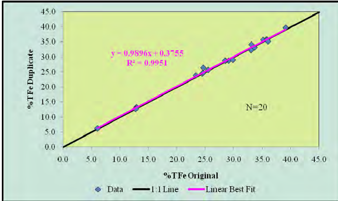
Figure 24. %TFe for preparation Duplicate vs. Original
