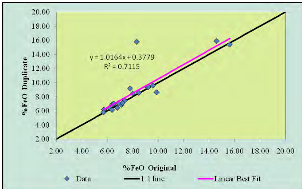
Figure 22. %FeO for Second Half Core Duplicate vs. Original
